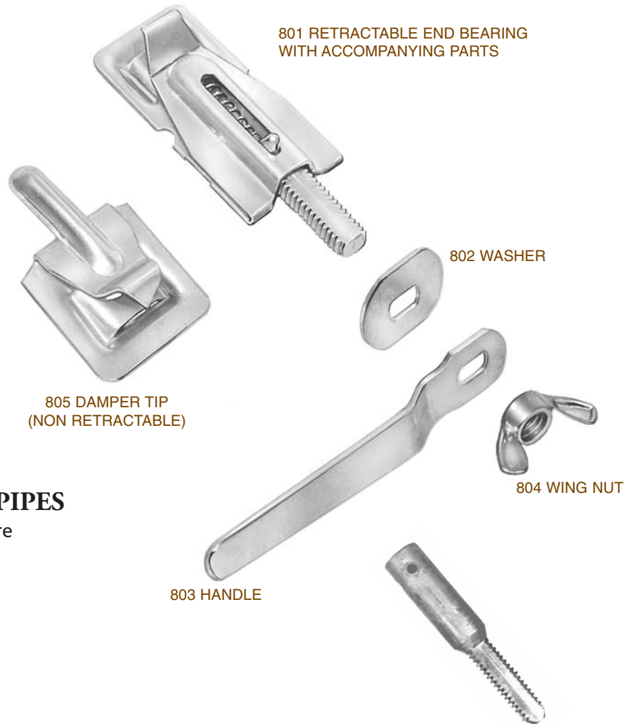
806 DAMPER EXTENSION FOR INSULATION
